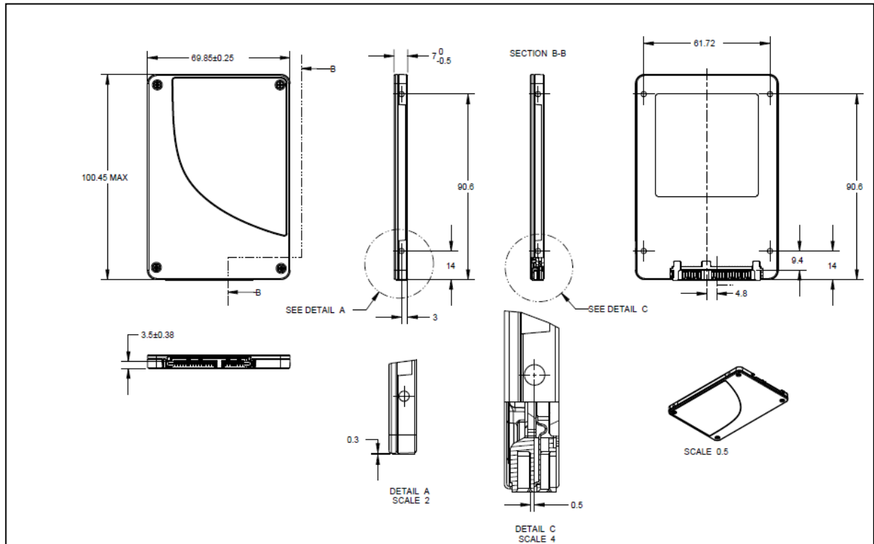
Figure 1: Intel SSD DC S3500 2.5-inch Dimensions
