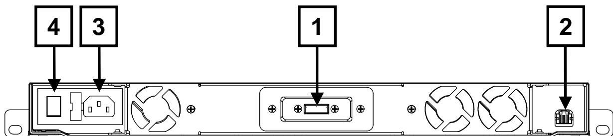
Figure. The rear of the StorageLoader with SAS drive.
