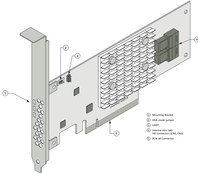
Figure 5 • Adaptec SmartRAID 3102E-8i
