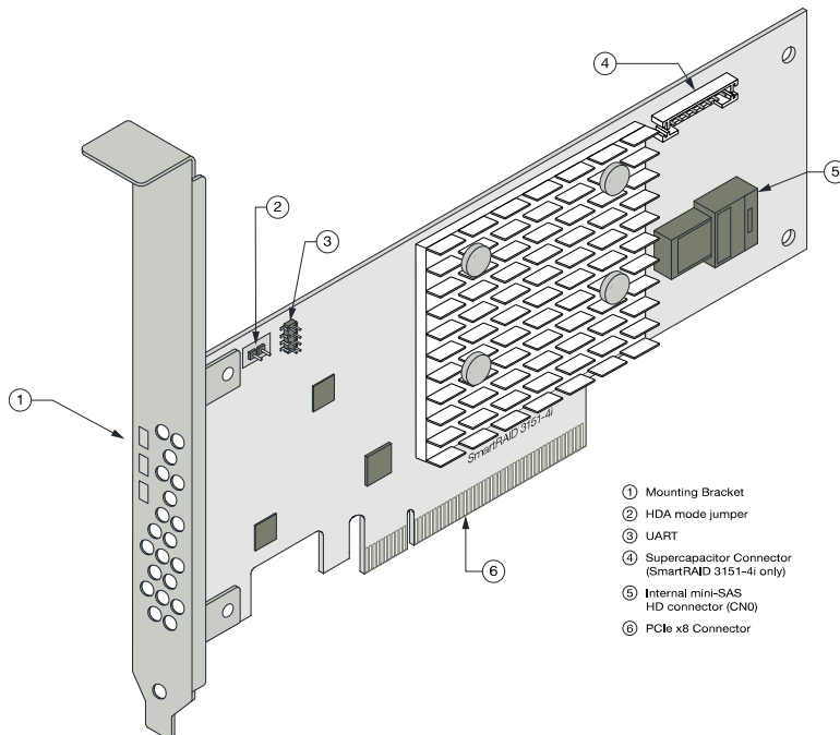
Figure 2 • Adaptec SmartRAID 31x1-4i
