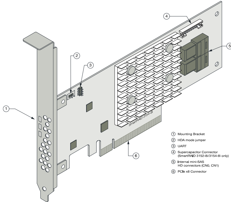
Figure 4 • Adaptec SmartRAID 31xx-8i
