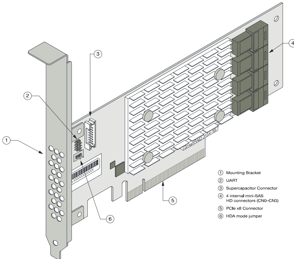
Figure 9 • Adaptec SmartRAID 3154-16i
