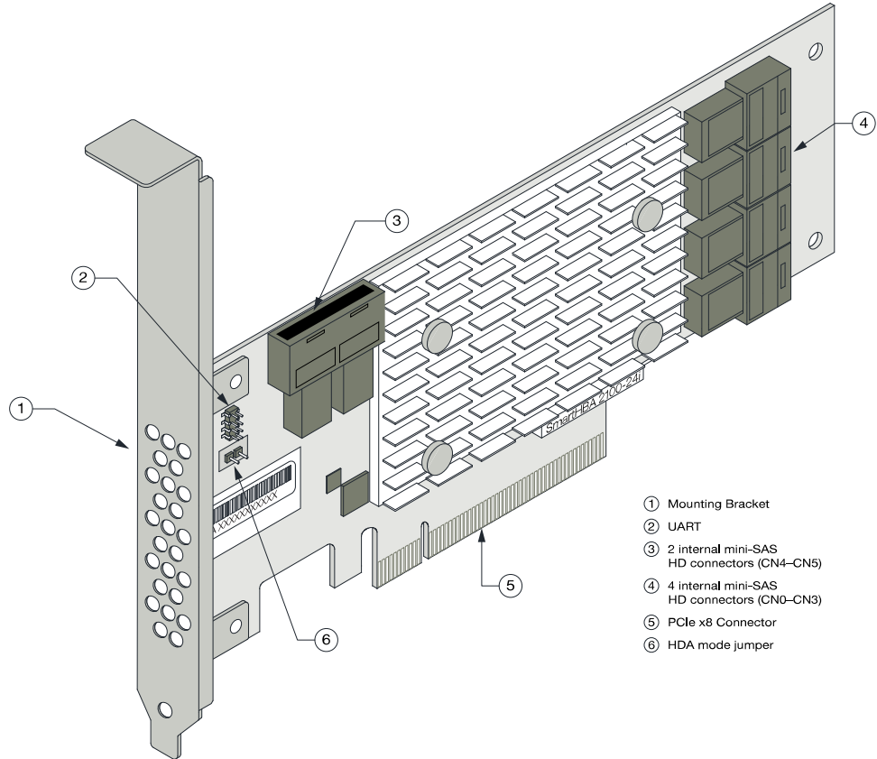
Figure 17 • Adaptec SmartHBA 2100-24i Features
