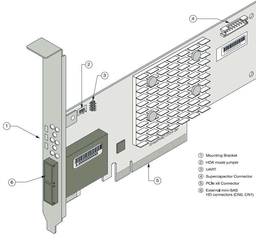
Figure 6 • Adaptec SmartRAID 3154-8e
