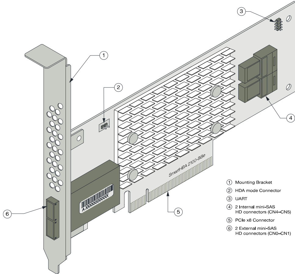
Figure 15 • Adaptec SmartHBA 2100-8i8e Features
