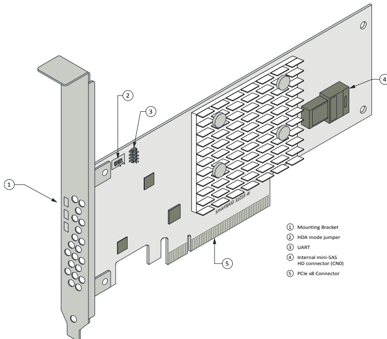
Figure 3 • Adaptec SmartRAID 3101E-4i
