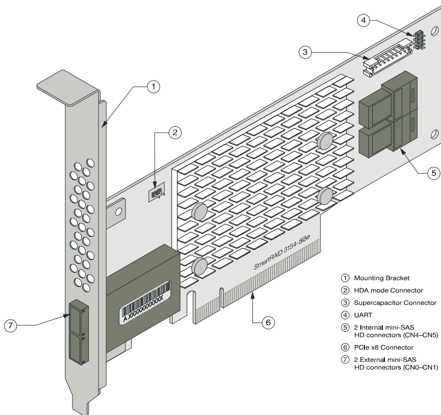
Figure 7 • Adaptec SmartRAID 3154-8i8e
