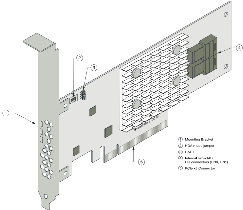
Figure 14 • Adaptec SmartHBA 2100-8i Features
