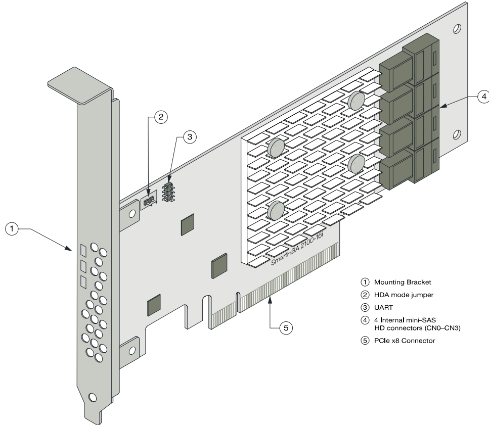
Figure 16 • Adaptec SmartHBA 2100-16i Features
