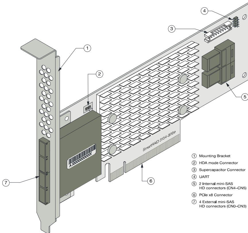
Figure 8 • Adaptec SmartRAID 3154-8i16e
