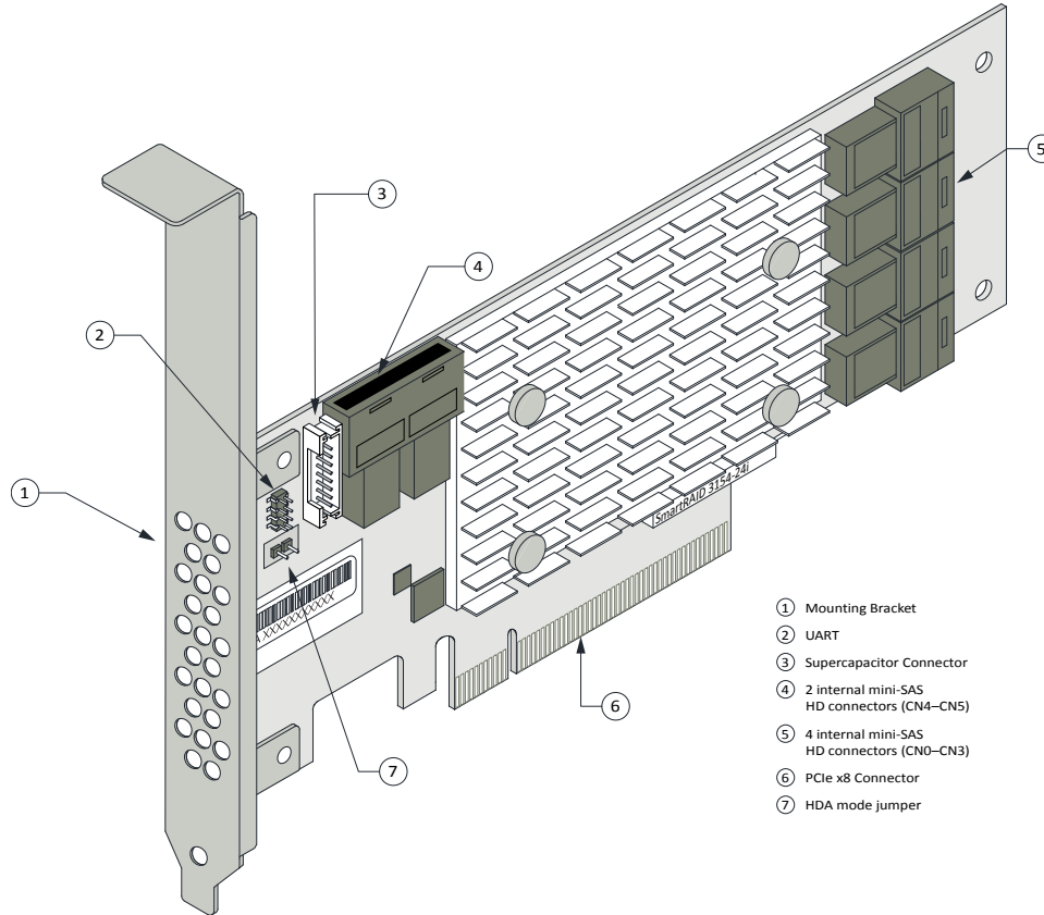
Figure 10 • Adaptec SmartRAID 3154-24i
