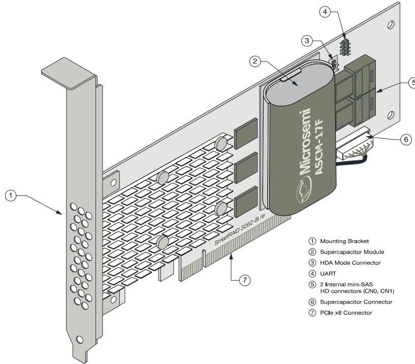
Figure 11 • Adaptec SmartRAID 3162-8i
