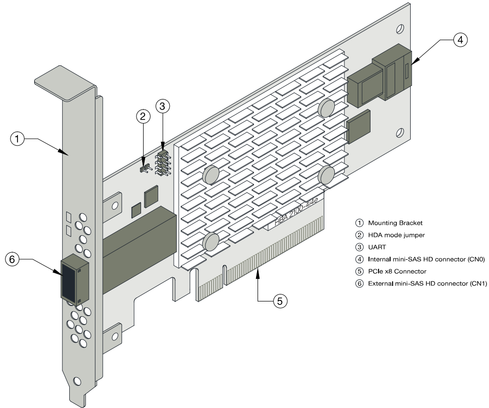
Figure 13 • Adaptec SmartHBA 2100-4i4e
