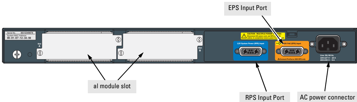
Figure 1-8. HP ProCurve 2910al-24G-PoE+ Switch
