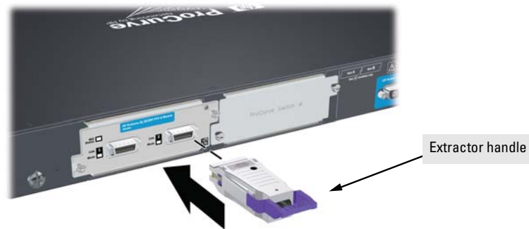
Figure 2-12. Installing an OMC
