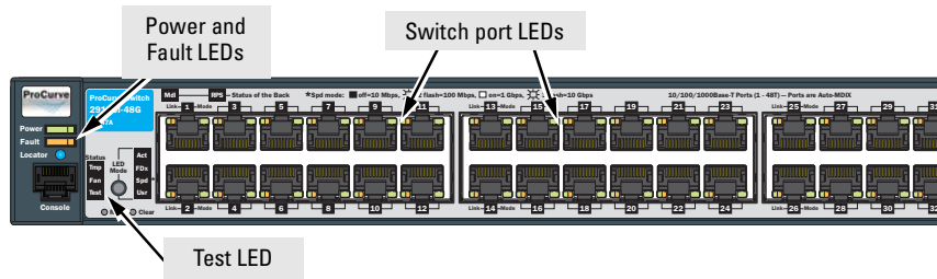
Figure 2-3. Checking the LEDs on the 2910al non-PoE switches
