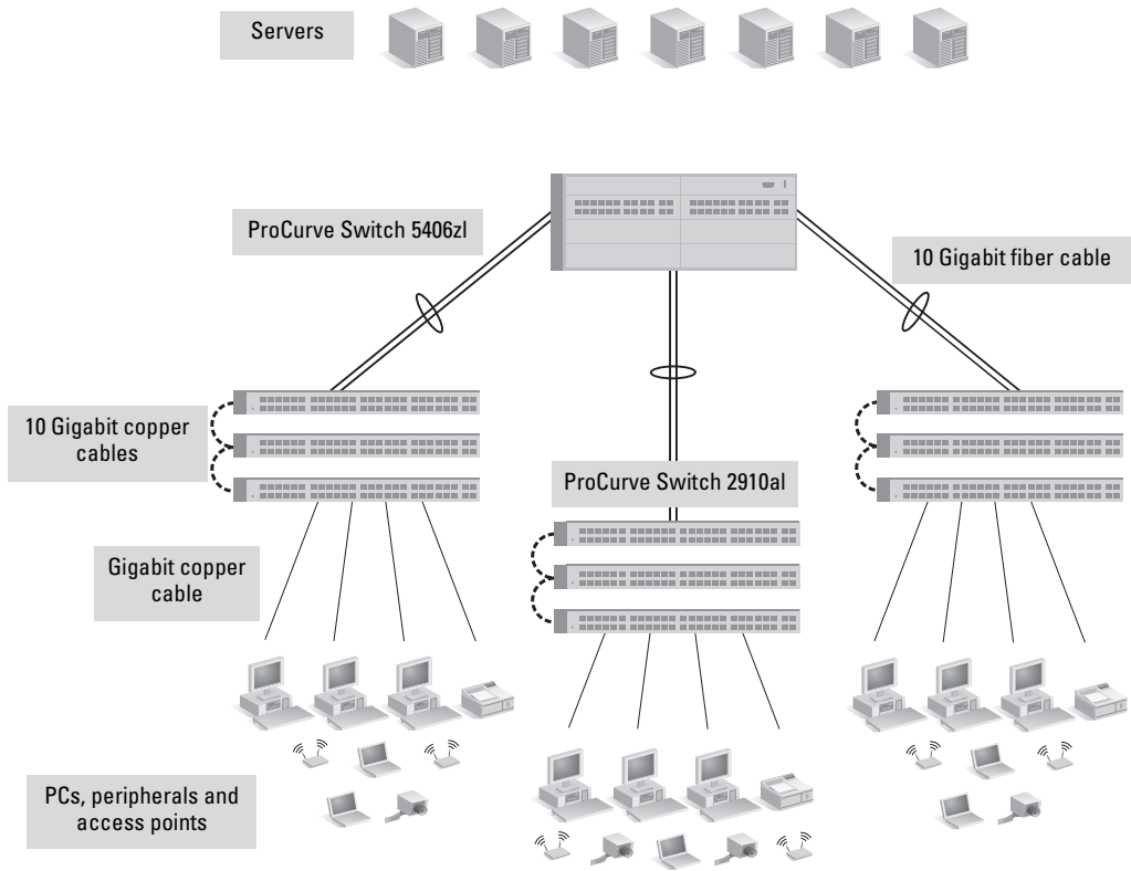
Figure 2-24. Example, PoE edge deployment
