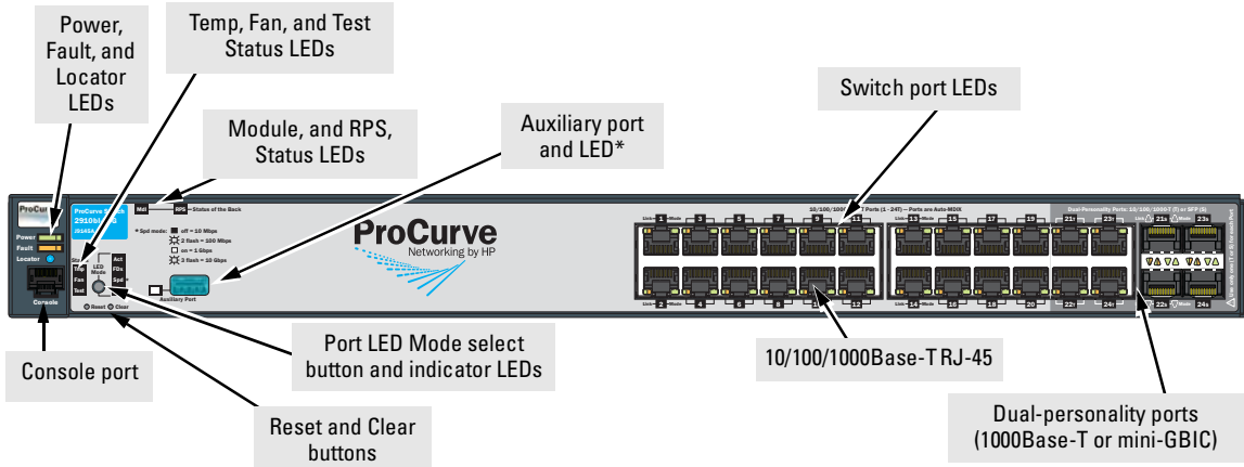
Figure 1-1. HP ProCurve 2910a1-24G Switch
