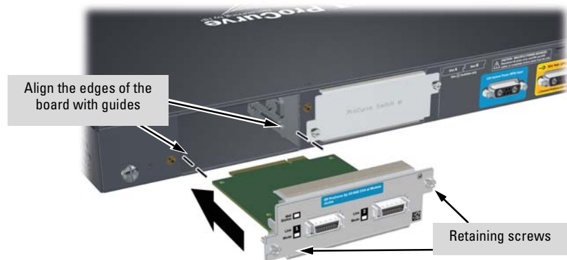
Figure 2-5. Installing a module
