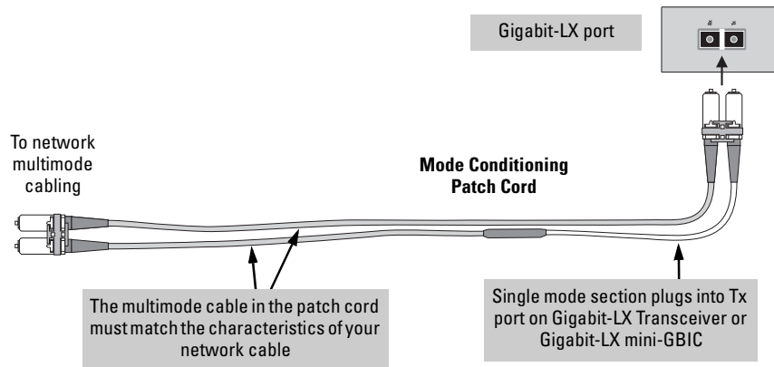
Figure C-1. Example: Connecting a Mode Conditioning Patch Cord for Gigabit-LX
