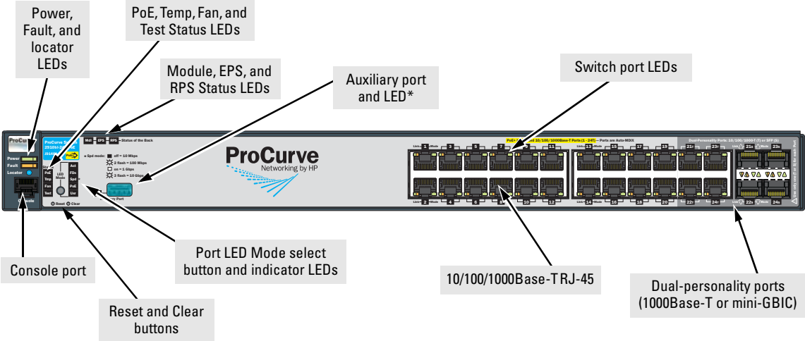
Figure 1-3. HP ProCurve 2910al-24G-PoE+ Switch
