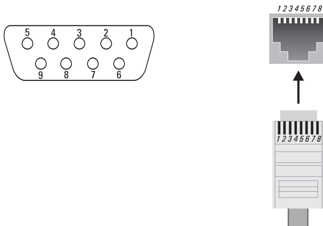
Figure 2-20. RJ-45 to DB-9 pinouts
