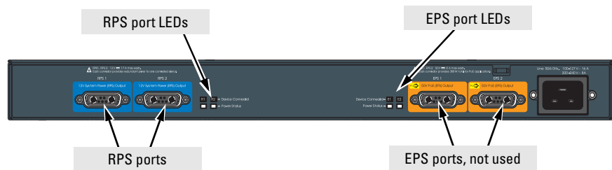
Figure 2-15. Back of 620 RPS/EPS
