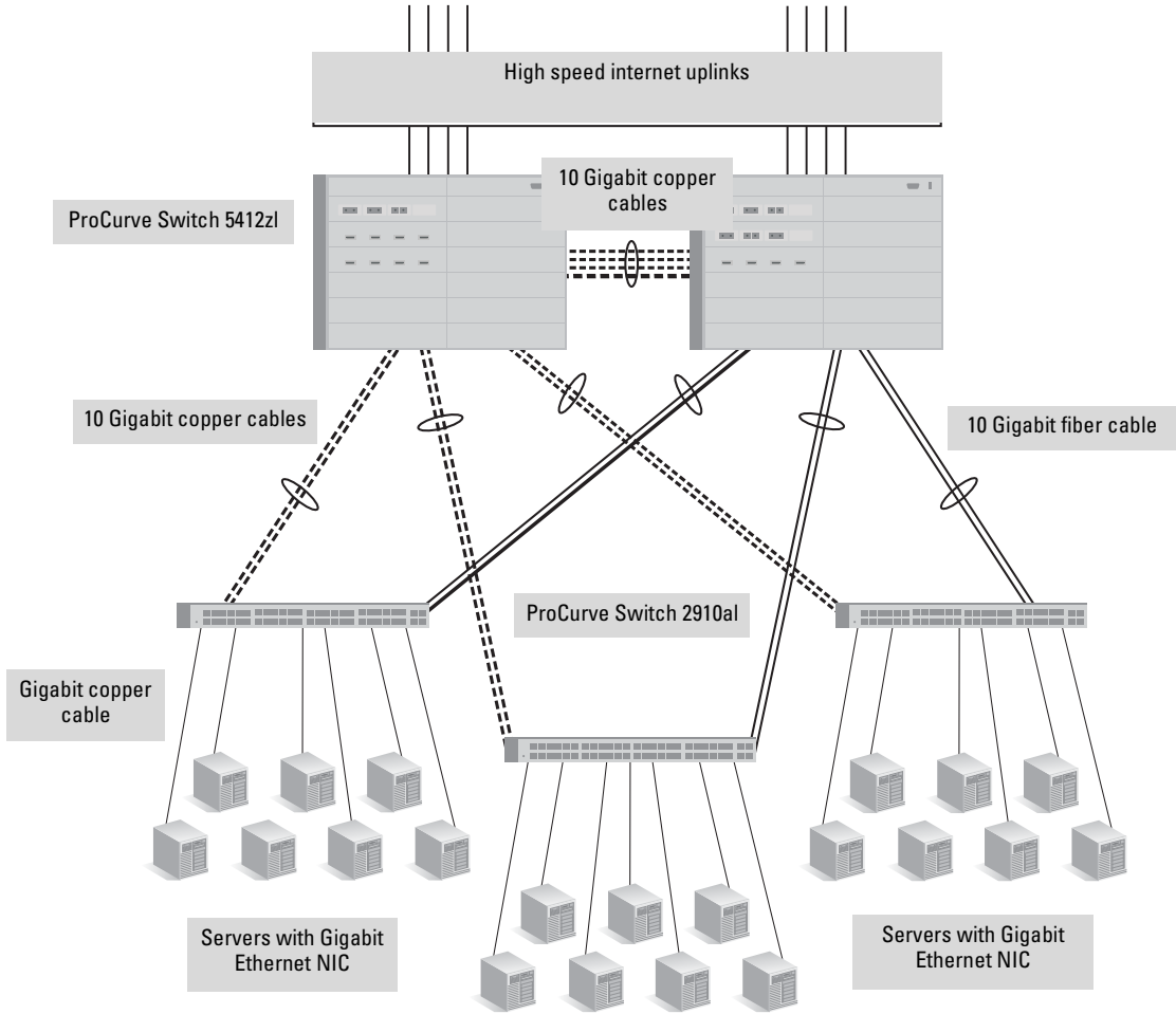
Figure 2-23. Example, server farm deployment
