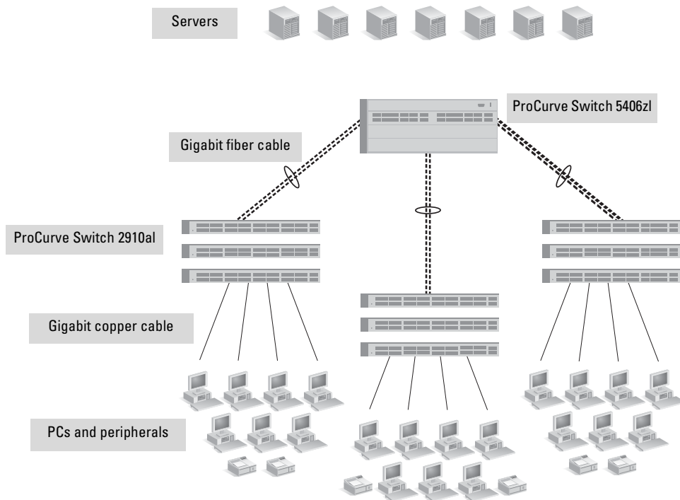
Figure 2-21. Example, gigabit edge deployment
