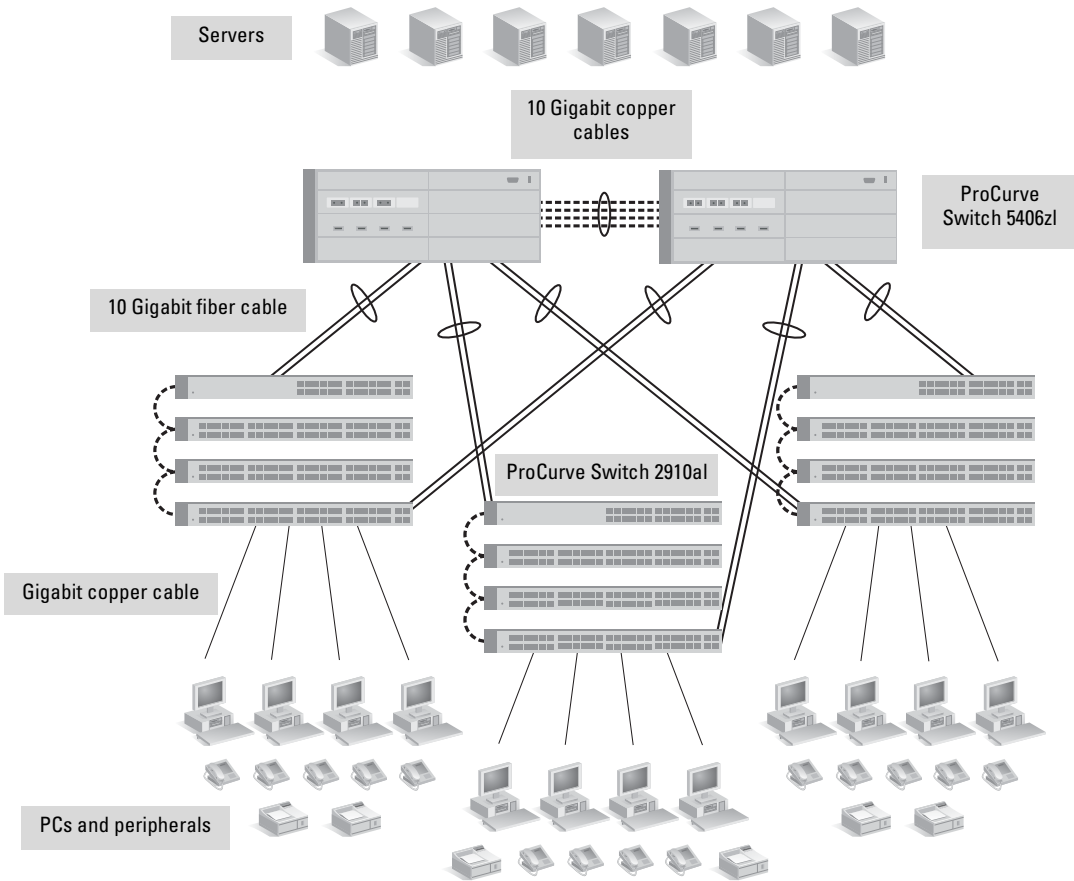
Figure 2-22. Example, high performance edge deployment
