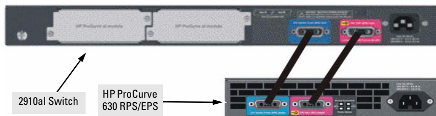
Figure 2-18. Connecting RPS/EPS to a switch
