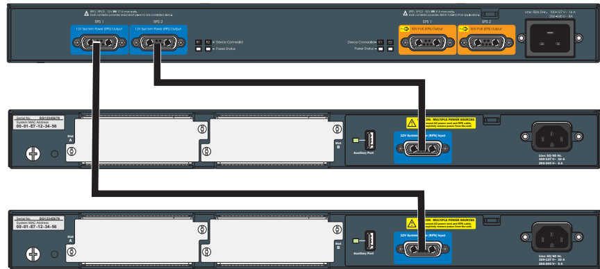
Figure 2-16. Connecting RPS to 2 switches
