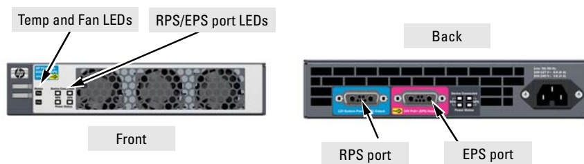
Figure 2-17. Front and Back of HP ProCurve 630 RPS/EPS
