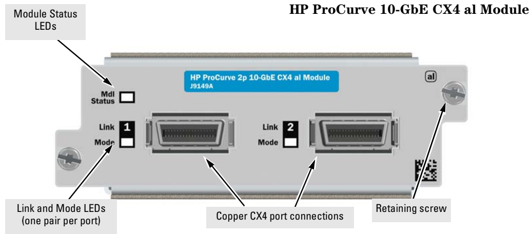
Figure 2. Front of the a1 10-GbE CX4 Module
