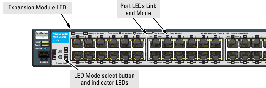
Figure 1-5. HP ProCurve 2910al-48G Switch
