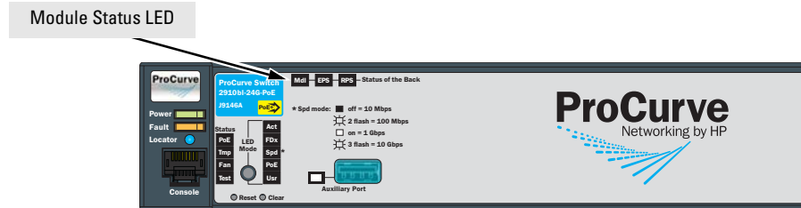
Figure 2-8. Location of Module Status LEDs
