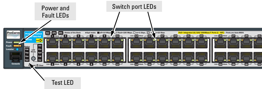
Figure 2-4. Checking the LEDs on the 2910al-PoE+ switches
