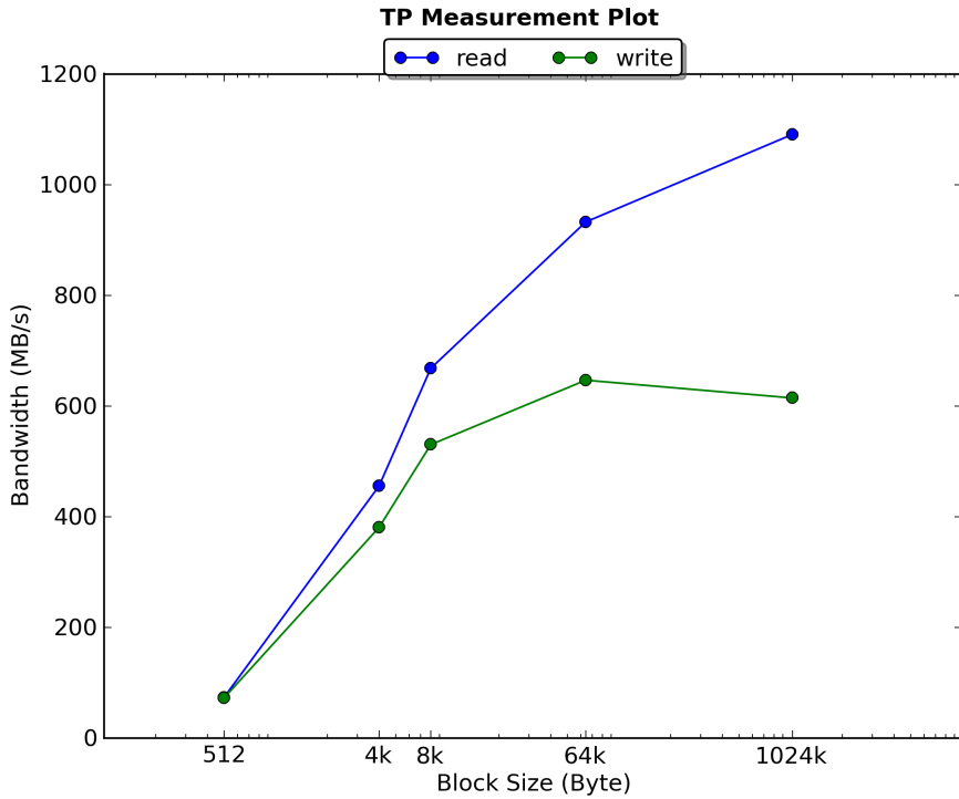
The Measurement Plot shows the average bandwidth of reads and writes in the measurement window. For all block sizes the seq. read and write bandwidth is plotted.
